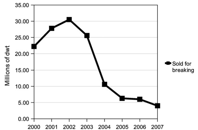
Fig. 6. Tonnage reported sold for breaking at the world level, 2000–2007 (millions of DWT). UNCTAD (United Nations Conference on Trade and Development), 2007.
